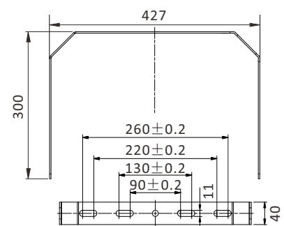
200W/240W/300W SBT-SL-L-SUS316
