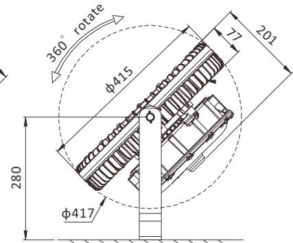
200W/240W/300W SBT-SL-L-SUS316
