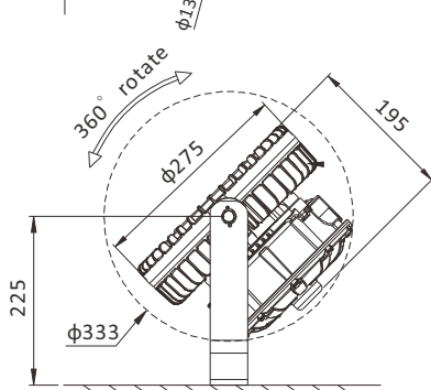
30W/45W/60W/80W SBT-SL-S-SUS316
