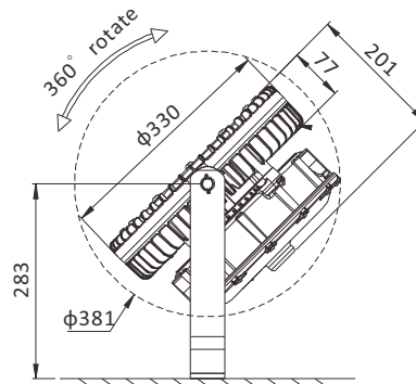
100W/120W/150W SBT-SL-M-SUS316
