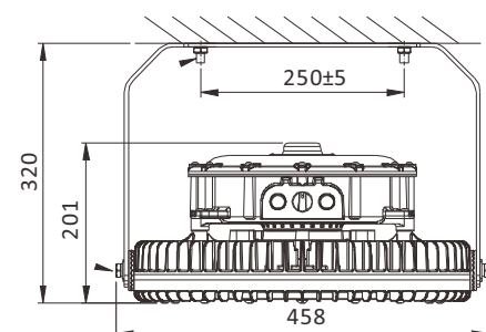
200W/240W/300W SBT-SL-L-SUS316
