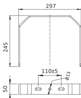
30W/45W/60W/80W SBT-SL-S-SUS316
