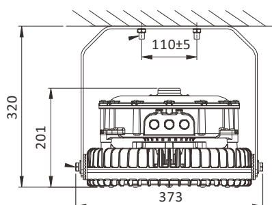
100W/120W/150W SBT-SL-M-SUS316
