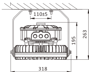
30W/45W/60W/80W SBT-SL-S-SUS316
