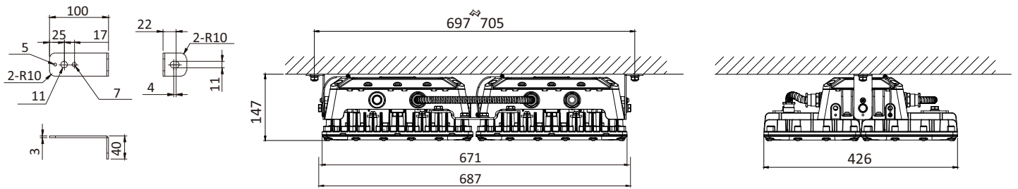
Ceiling mount
