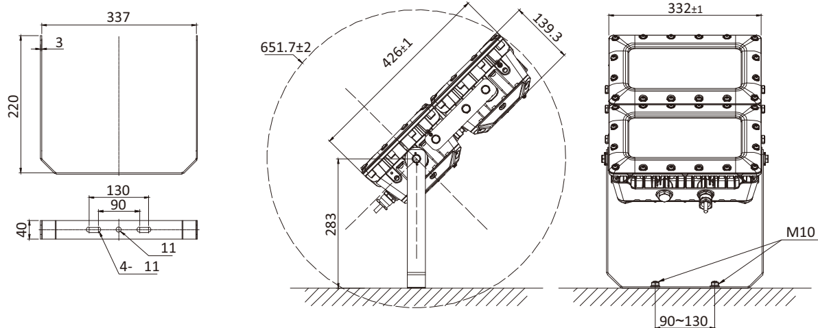
Stanchion mount / Wall mount
