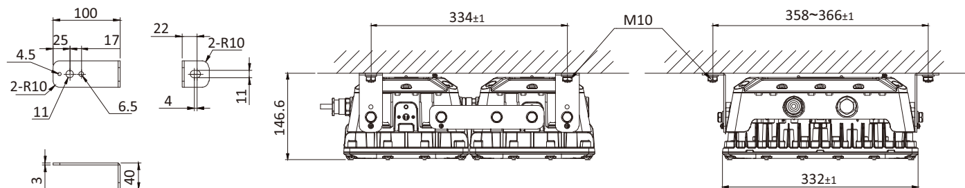
Stanchion mount / Wall mount
